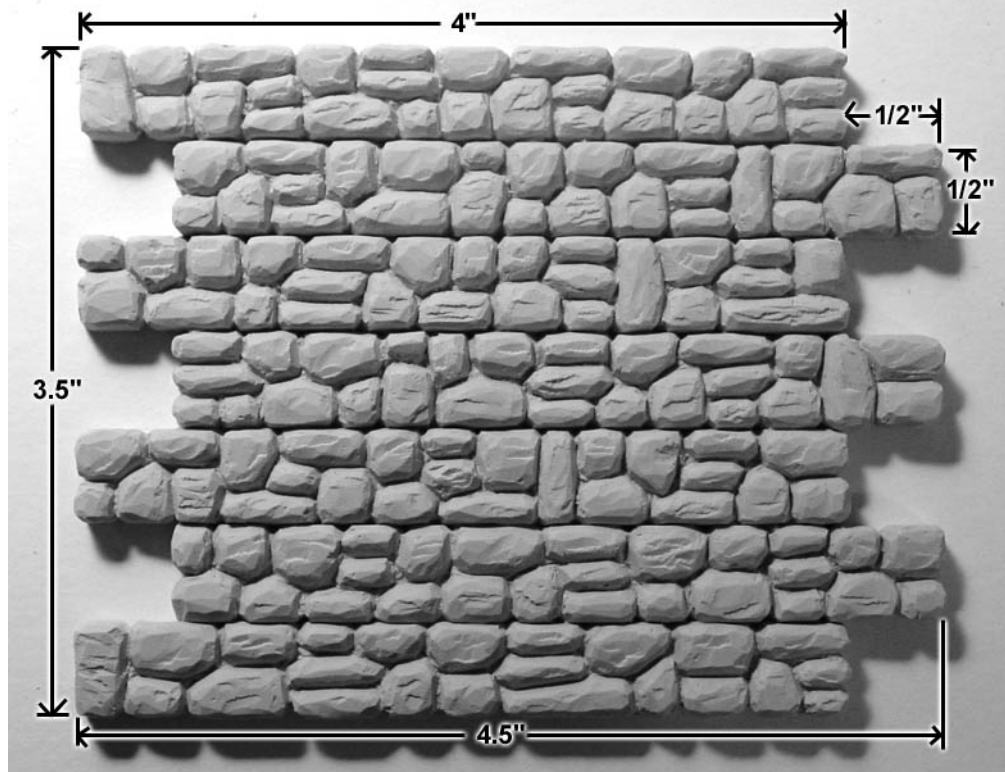
Mold #261 Piece Block is 1/4" thick. Block shown actual size.
