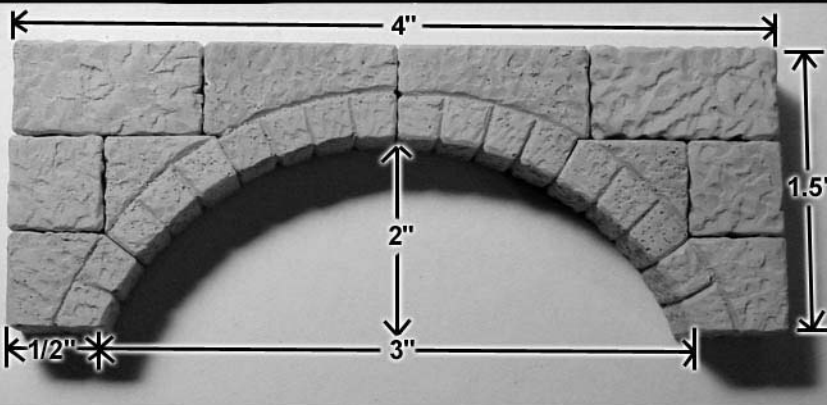
Arch Details
